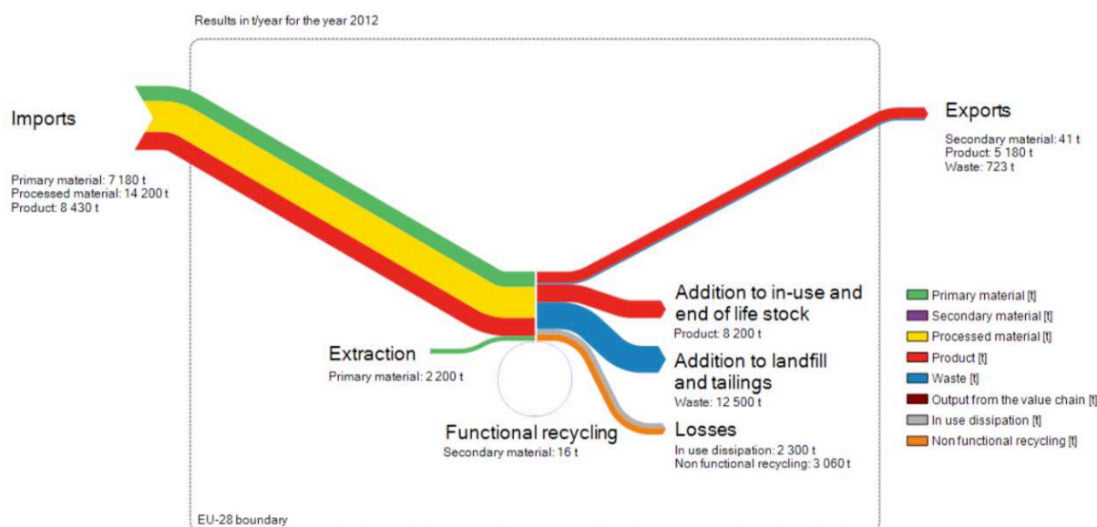
Figure 3.8 Simplified lithium material flows in LCE in Europe for 2012 (Deloitte, 2015)
