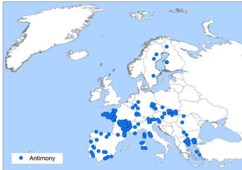
Figure 3.1 Antimony occurrence in Europe (SCRREEN, 2018)
