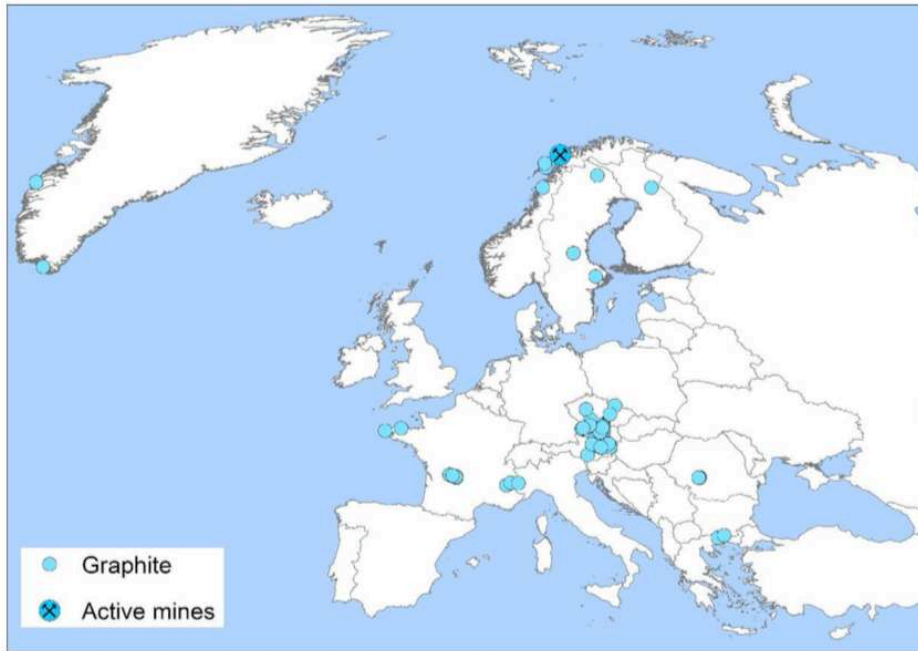
Figure 3.12 Active mine and occurrences of natural graphite in Europe (SCREEN, 2018)
