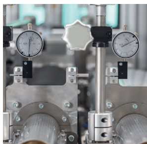
Engraved roller system
